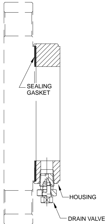
Figure 4.6 – LD300L- Sealing Gasket
