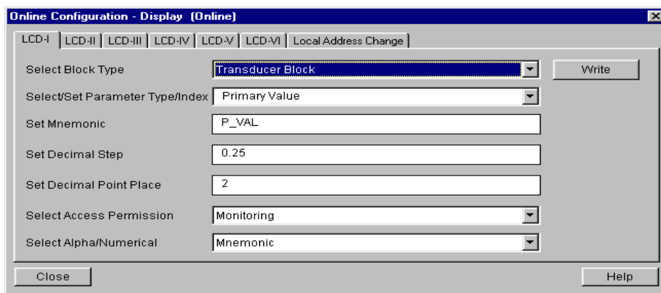
Figure 3.34 – Display Block
