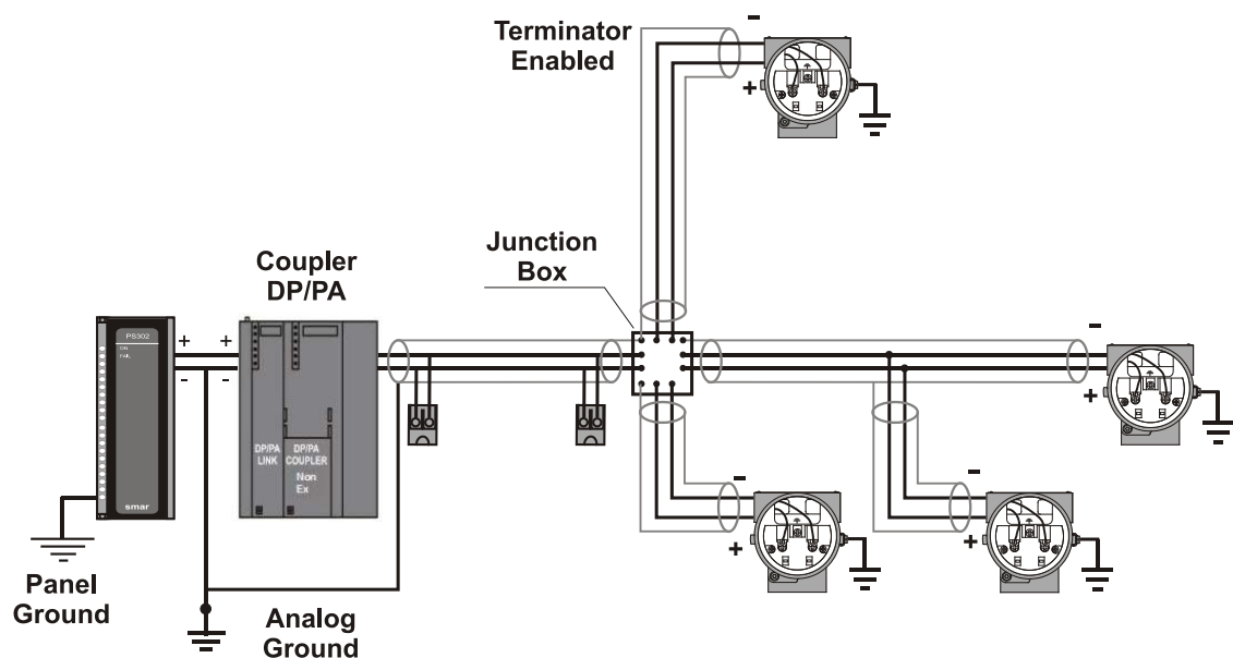
Figure 1.10 - Tree Topology
