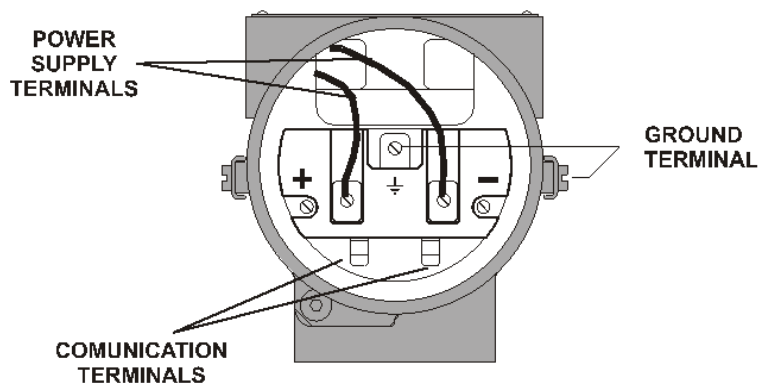
Figure 1.6 - Terminal Block
