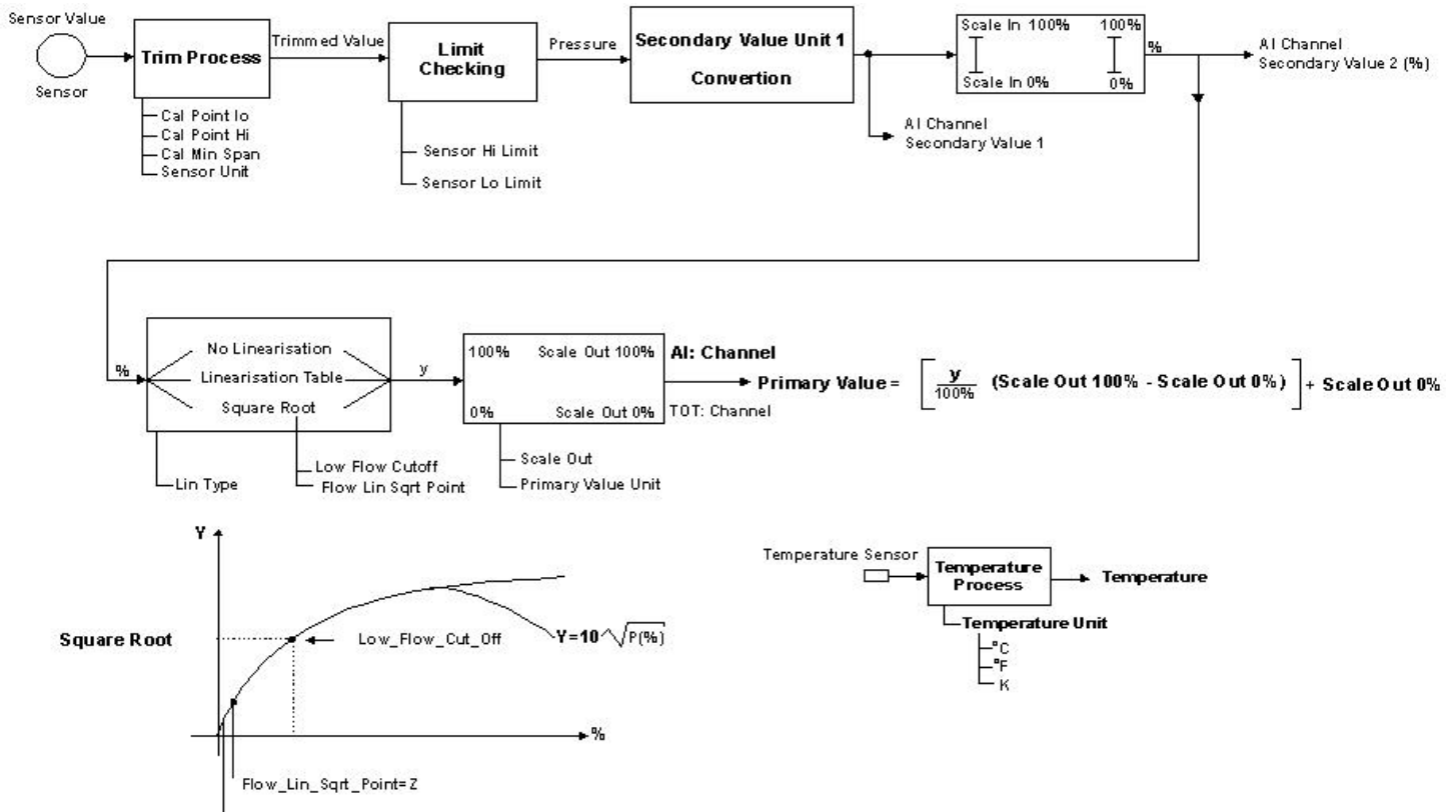
Figure 3.1 – Transducer Block Diagram
