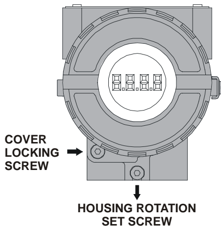
Figure 1.4 - Housing Rotation Set Screw
