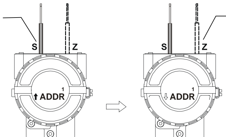
Figure 3.46 - Step 6 - LD303
