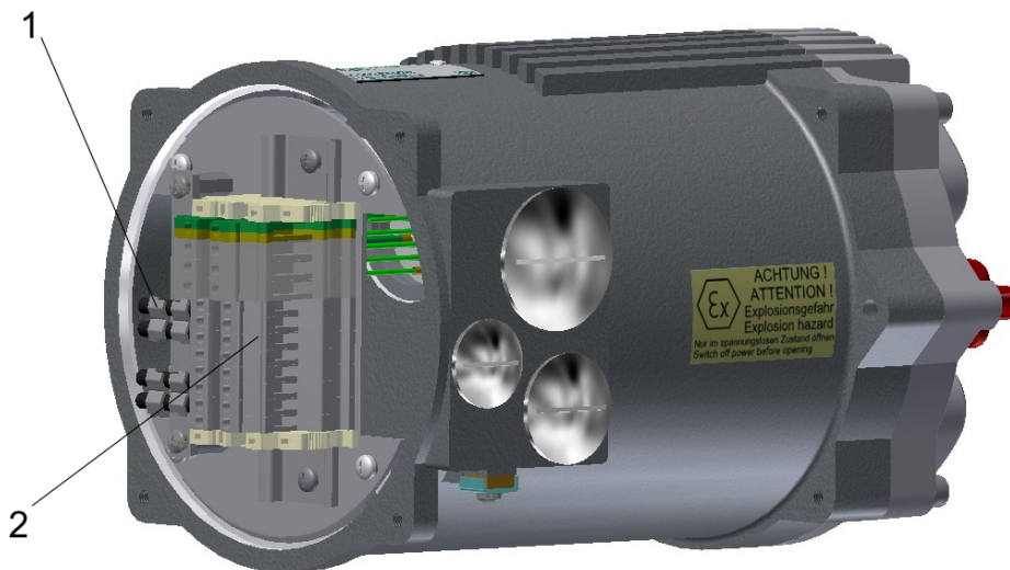
Figure 7: 1... shielding connection clamp, 2... terminal strip
